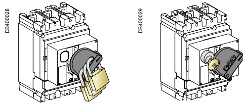
Rotary-handle locking using a padlock or a keylock.
